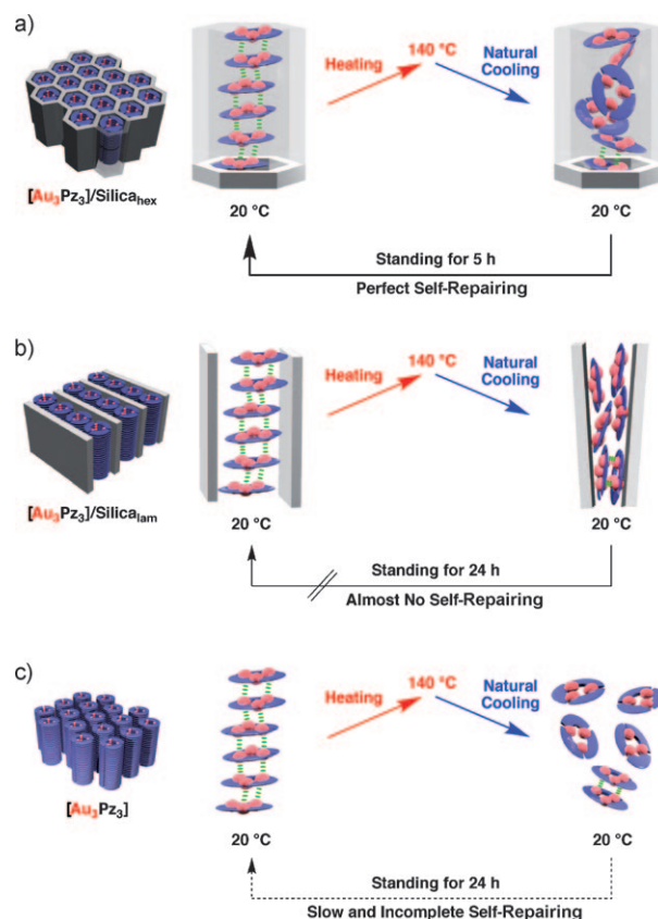
Figure 5. Schematic representations of the effects of heating on columnar assembled [Au 3 Pz 3 ] confined within a) silicate nanochannels ([Au 3 Pz 3 ]/silica hex ), b) silicate layers ([Au 3 Pz 3 ]/silica lam ), and c) in the absence of silica as a reference.
