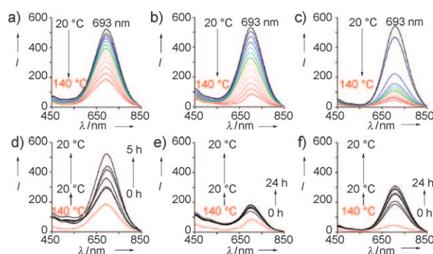
Figure 3. Luminescence spectral changes ( \lambda_{\text{ext}} = 276 nm) of a,d) [\text{Au}_3\text{Pz}_3]/\text{silica}_{\text{hex}} , b,e) [\text{Au}_3\text{Pz}_3]/\text{silica}_{\text{lam}} , and c,f) bulk [\text{Au}_3\text{Pz}_3] on stepwise heating from 20 to 140^\circ\text{C} (red curve in (a)–(c)) and subsequent natural cooling from 140 to 20^\circ\text{C} , then being held at the same temperature for 24 h (black curves in (d)–(f)).
